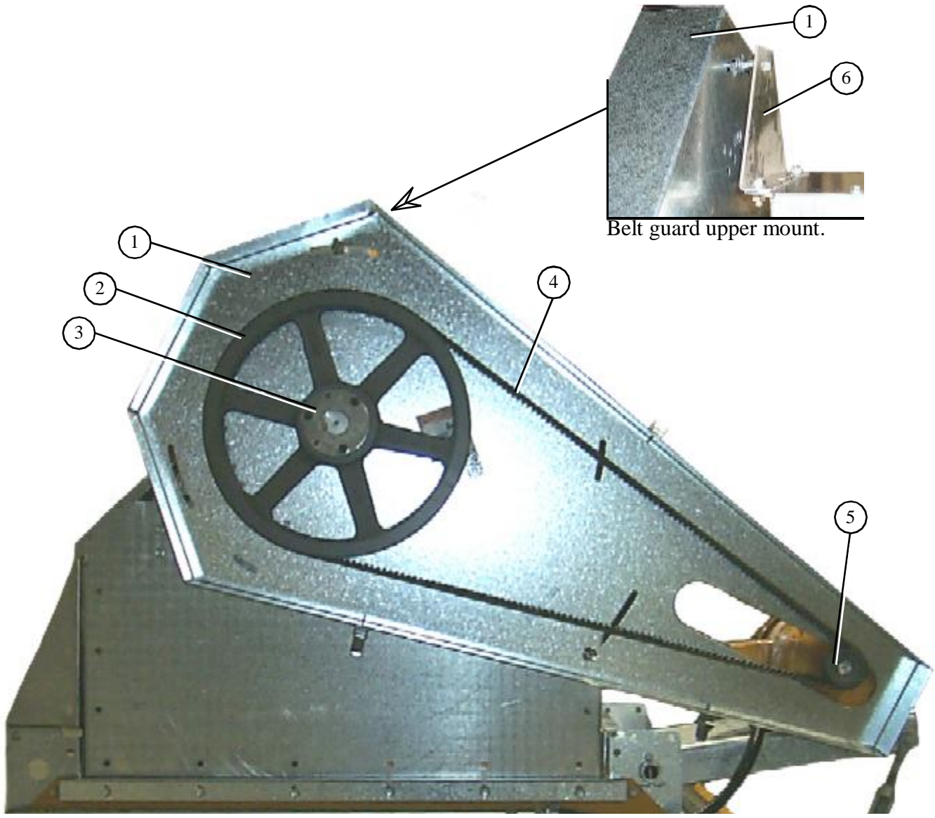
Top Auger drive components.
